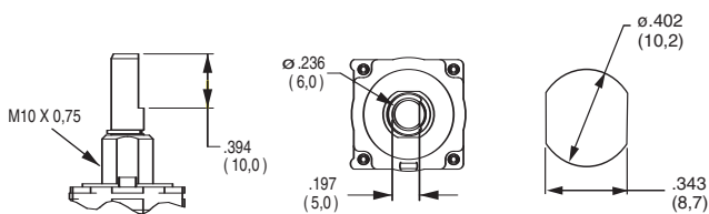
F METRIC SHAFT WITH FLAT 0.236 (6,0)
