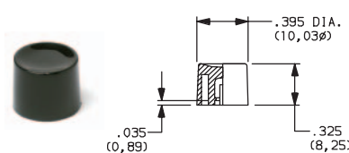
Cap Compatible with 13-19 actuators
