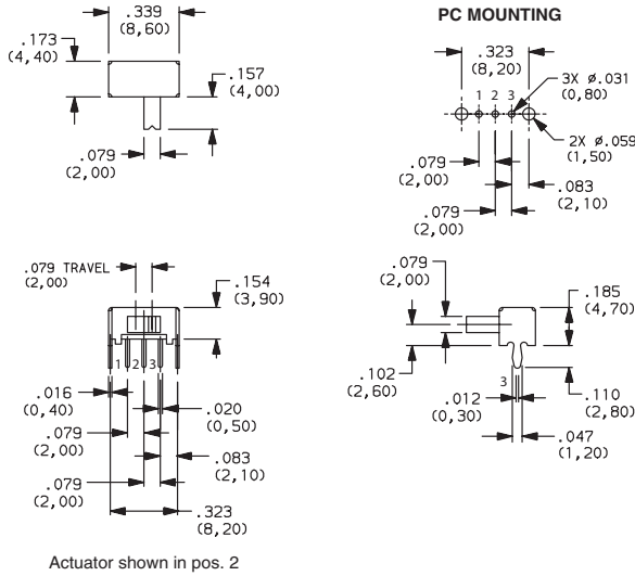
OS102011MA1QN1 SPDT
