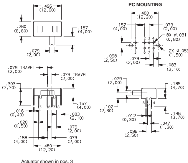
OS203011MA2QP1 DP3T
