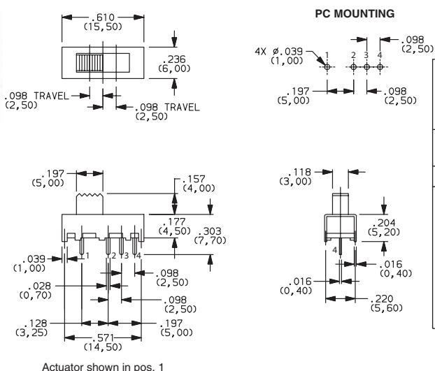
OS103012MU2QP1 SP3T
