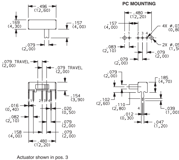
OS103011MA7QP1 SP3T
